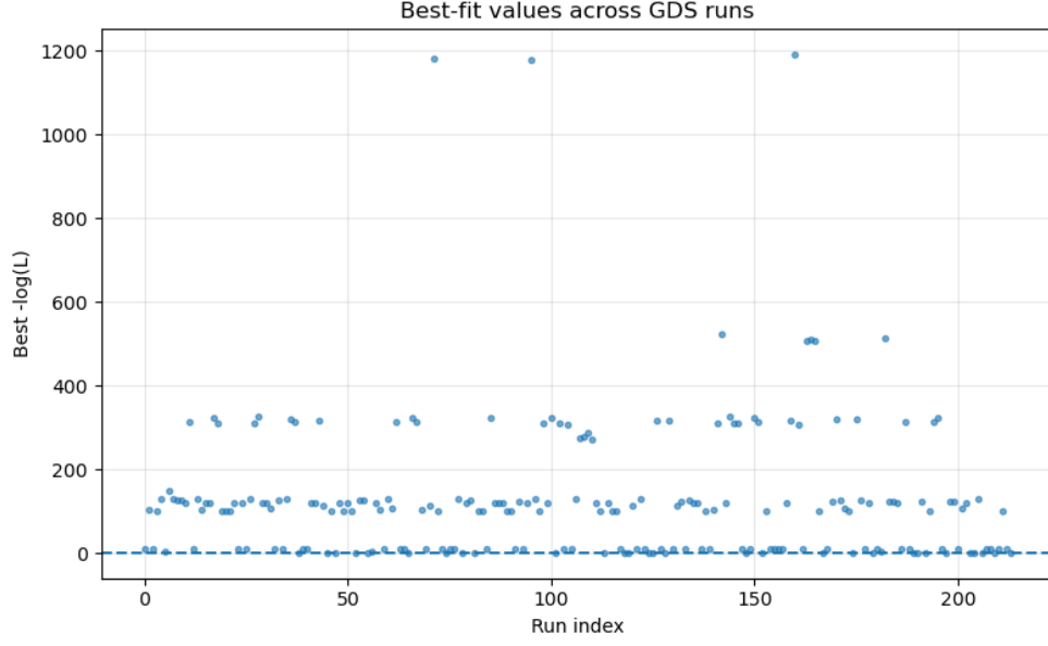
Figure 2: Best-fit likelihood values across independent GDS runs. The presence of consistently low values indicates stable minima, while higher values correspond to exploratory regions of the parameter space.
