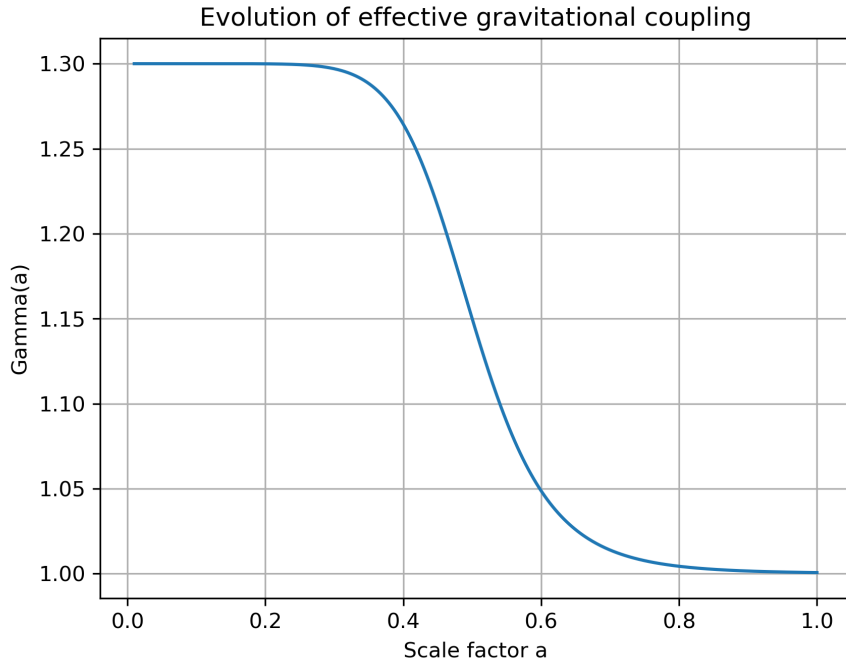
Figure 3: Evolution of the effective gravitational coupling \Gamma(a) .
