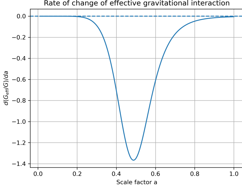
Figure 7: Rate of change of the effective gravitational interaction. The negative values indicate that the effective gravitational strength decreases as the Universe evolves.
