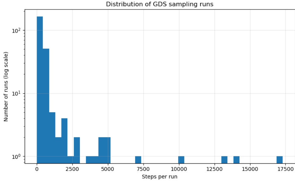
Figure 1: Distribution of sampling depth across GDS runs. The multi-scale structure reflects the adopted strategy of exploratory scans, targeted refinements, and confirmatory runs.
