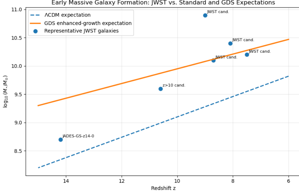
Figure 6: Stellar mass as a function of redshift for representative early galaxies. The dashed \Lambda CDM curve illustrates a schematic standard expectation for early galaxy assembly, while the solid GDS curve shows enhanced early growth. JWST points are shown schematically for illustrative comparison. The plotted observational points are illustrative and intended to highlight qualitative trends rather than provide a precise statistical fit.
