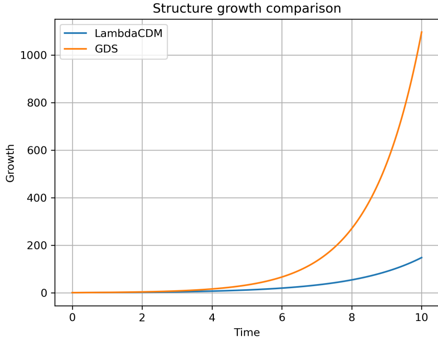
Figure 4: Illustrative comparison of structure growth between GDS and \Lambda CDM. The presented plots are illustrative and do not represent results from full cosmological simulations.
