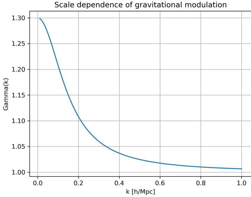
Figure 5: Scale dependence of the modulation function \Gamma(k) .
